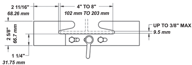
#015-698 BEAM CLAMP
