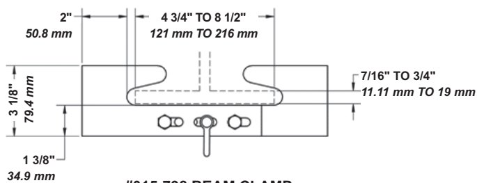
#015-798 BEAM CLAMP
