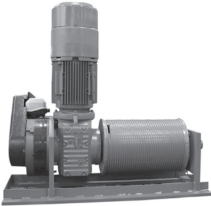
Drum Hoist
